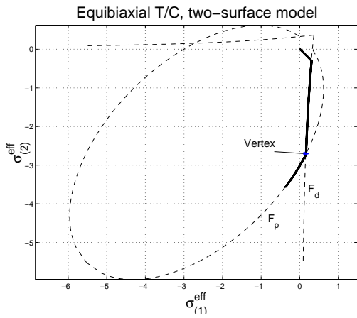
Figure 10: Equibiaxial T/C, associated flow - stress path
