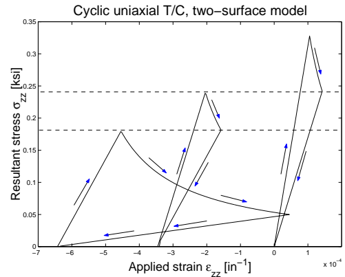
Figure 6: Cyclic uniaxial tension/compression - (a) Total response, (b) Tensile stress \sigma_{zz} close-up
