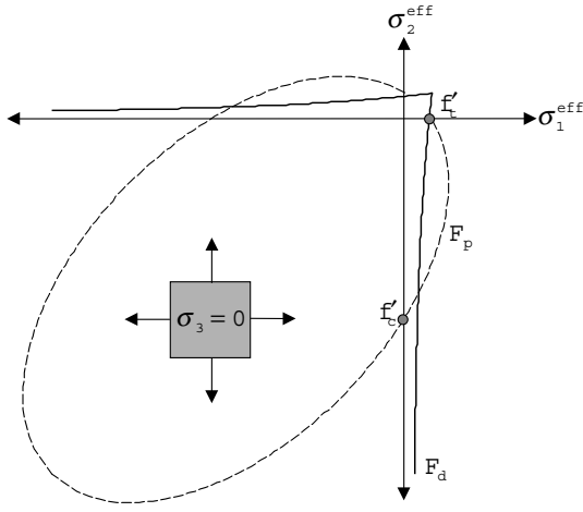
Figure 2: Plane stress envelope for the two-surface model
