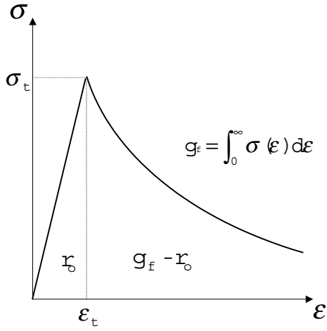
Figure 1: Uniaxial stress-strain curve defining r_o , g_f
