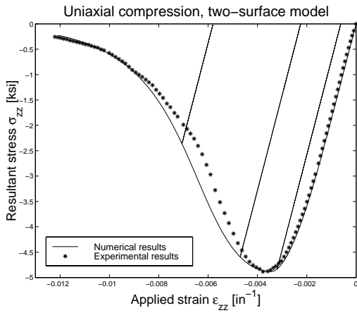
Figure 4: Uniaxial compression, two-surface model, unconfined compression
