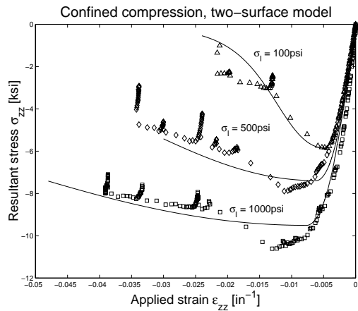
Figure 5: Uniaxial compression, two-surface model, confined compression
