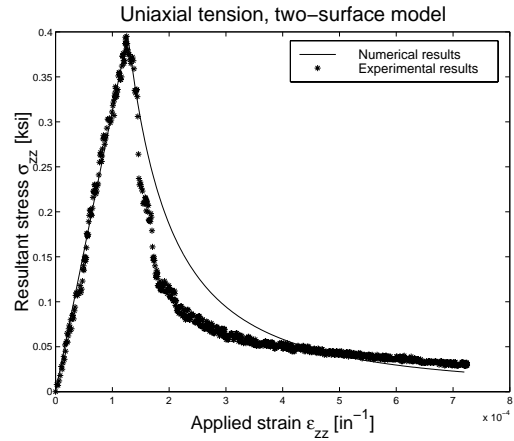
Figure 3: Uniaxial tension, two-surface model
