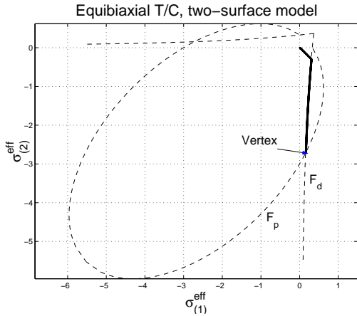
Figure 8: Equibiaxial T/C, non-associated flow - stress path
