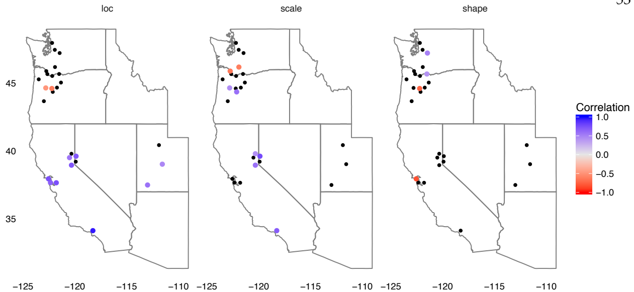
Figure 3.2: Regional mean correlations between nonstationary GEV parameter estimates for peak 3-day total flow with peak 3-day total rainfall from surrounding rain gages. Each point indicates the approximate location of a basin outlet and a colored point indicates the strength of the correlation, with black points indicating no significant relationship.
