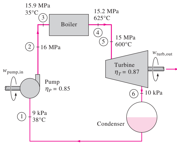
FIGURE 42 Schematic and T - s diagram for Example 8.
