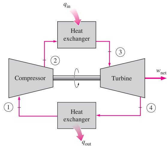
FIGURE 26 A closed-cycle gas-turbine engine.
